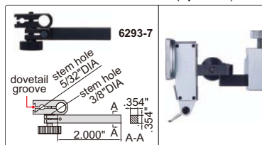
dial test indicator holder (optional)
