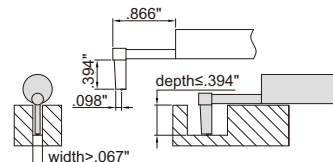
deep groove probe (optional), Part No. ISR-C002-DGP
