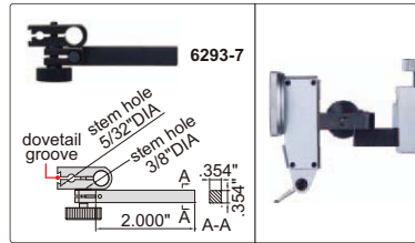
dial test indicator holder (optional)
